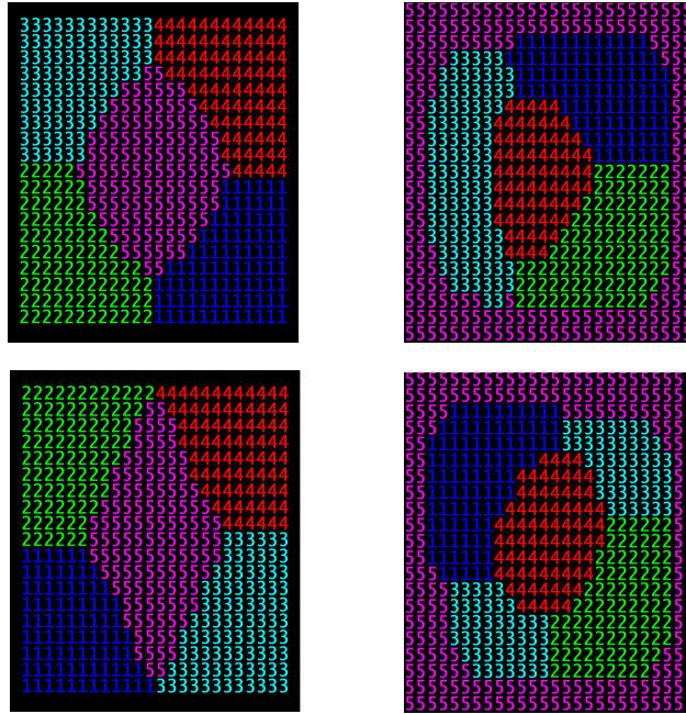
Figure 4: Twist and twin defects in normal neighbors patterns (computed on a square lattice). Top left: Correct pattern for Figure 3. Bottom left: Stable local minimum with inconsistent handedness. Top right: Correct pattern for a related adjacency graph particularly prone to stable twinning; boundary conditions fixed at 5. Bottom right: Twinned configuration.
