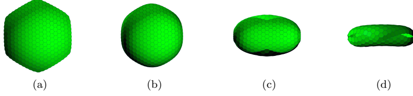
Figure 6: Uniform disc subject to extrinsic curvature such as due to apical/basal constriction, showing spontaneous cylindrical buckling beyond a certain critical curvature. Curvature set-points of (a) 100mrad/cell, (b) 200mrad/cell, (c) 300mrad/cell, (d) 400mrad/cell. Substrate stiffness k_B = 0.8 .
